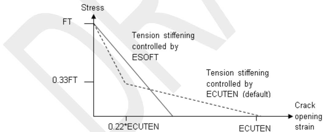
Tensile Behaviour of Concrete
