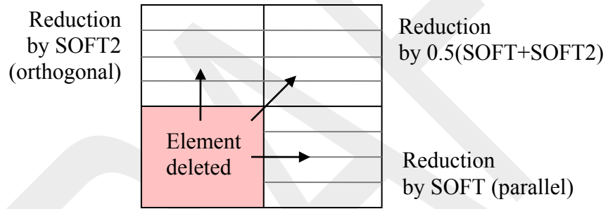
Figure 54.2 Direction dependent softening
