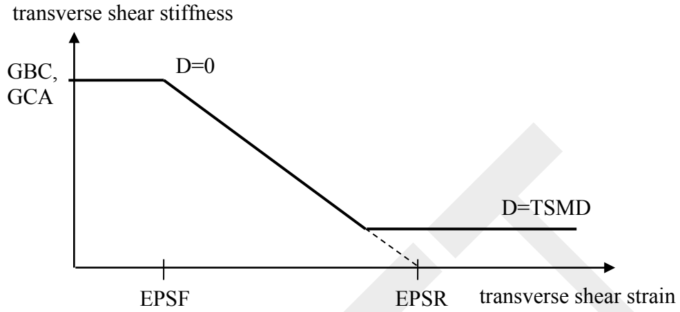
Figure 54.1 Linear damage for transverse shear behavior
