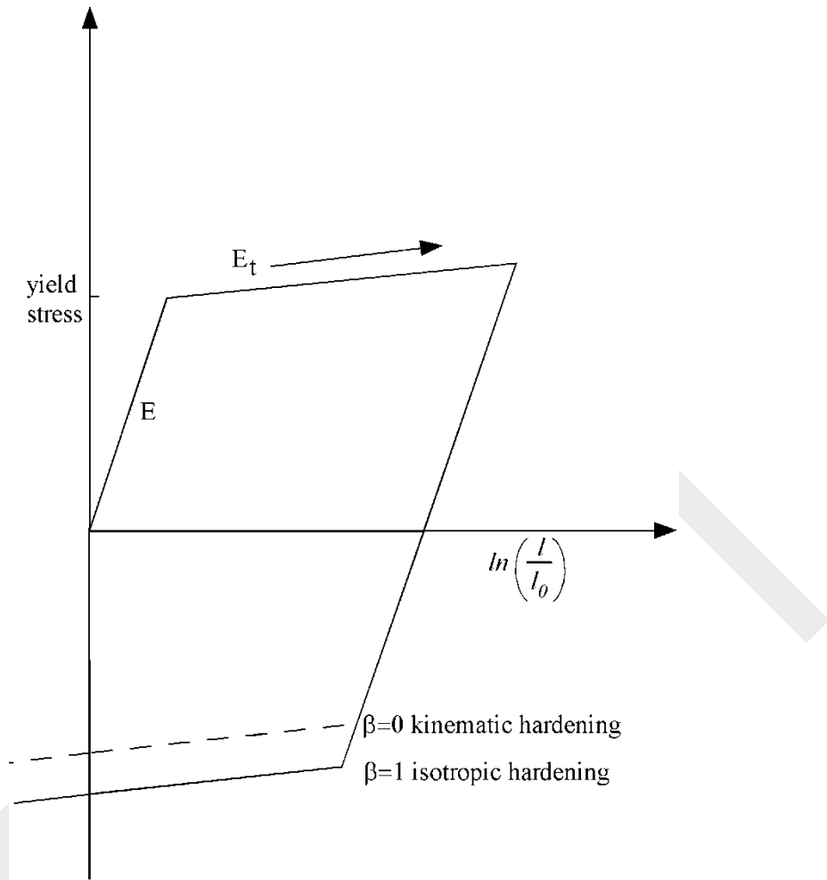
Figure 3.1. Elastic-plastic behavior with kinematic and isotropic hardening where l_0 and l are undeformed and deformed lengths of uniaxial tension specimen. E_t is the slope of the bilinear stress strain curve.
