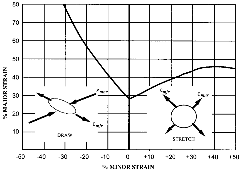
Figure 39.1. Forming Limit Diagram.
