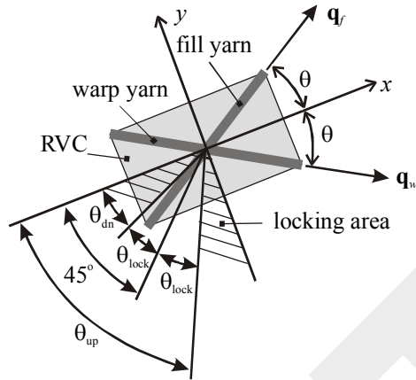
Fig. 3. Locking angles.
