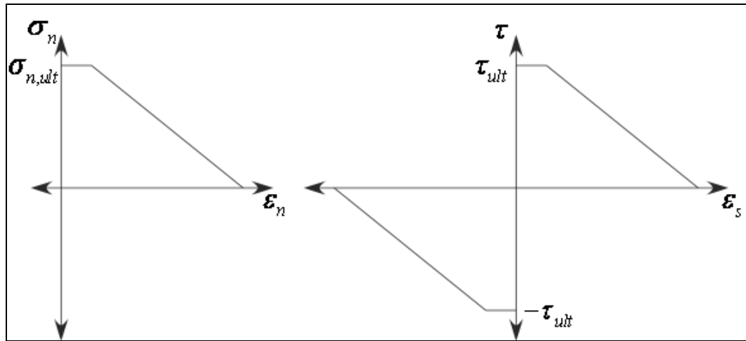
Figure 132.1. Shows stress bounds for the active normal component (left) and the archite shear component (right).
