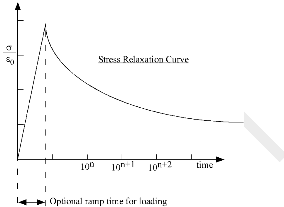
Figure 76.1. Relaxation curve. This curve defines stress versus time where time is defined on a logarithmic scale. For best results, the points defined in the load curve should be equally spaced on the logarithmic scale. Note the values for the abscissa are input as time, not log(time). Furthermore, the load curve should be smooth and defined in the positive quadrant. If nonphysical values are determined by least squares fit, LS-DYNA will terminate with an error message after the initialization phase is completed. If the ramp time for loading is included, then the relaxation which occurs during the loading phase is taken into account. This effect may or may not be important.
