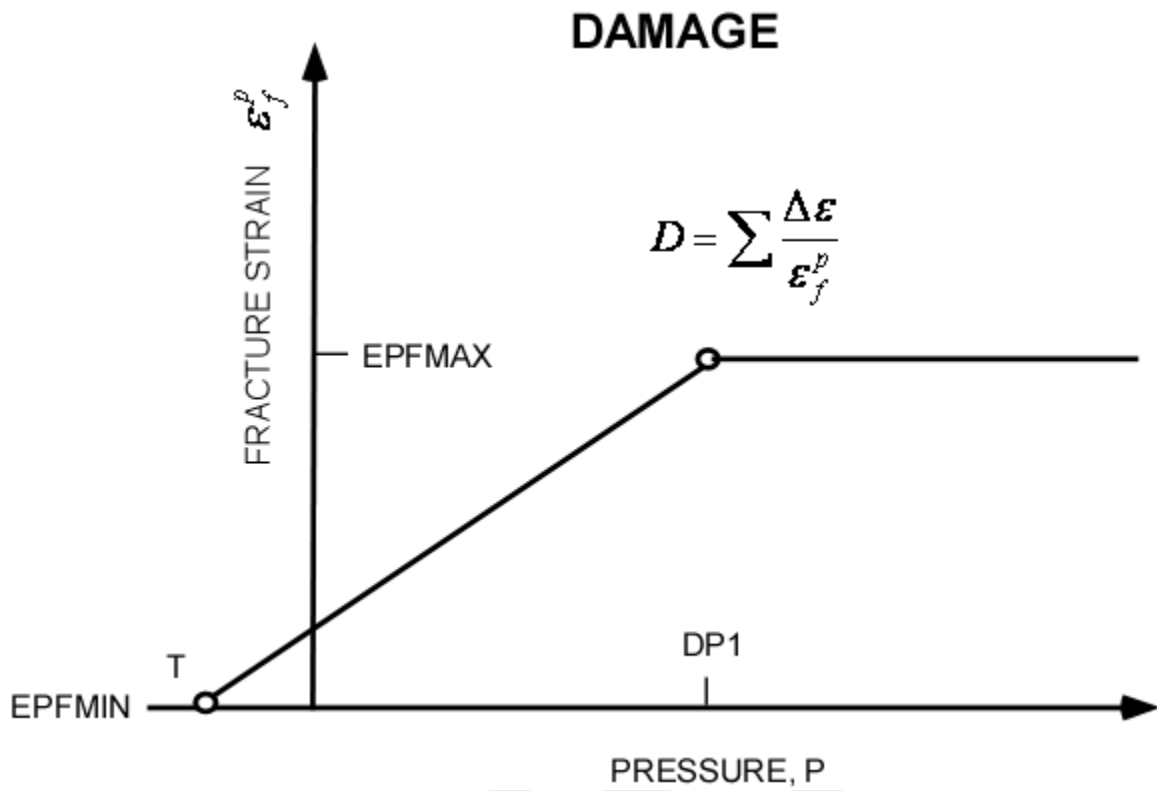
Figure 241.2. Fracture strain versus pressure.
