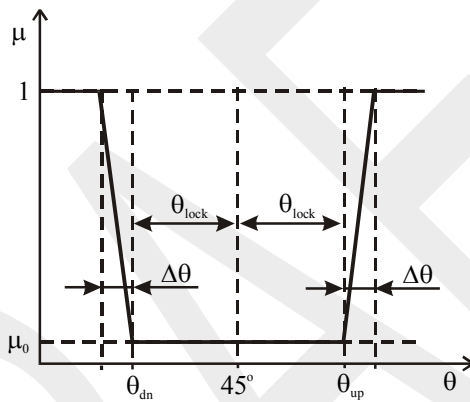
Fig. 4. Discount factor as a function of braid angle, \theta .
