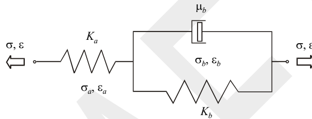
Fig. 2. Three-element viscoelasticity model
