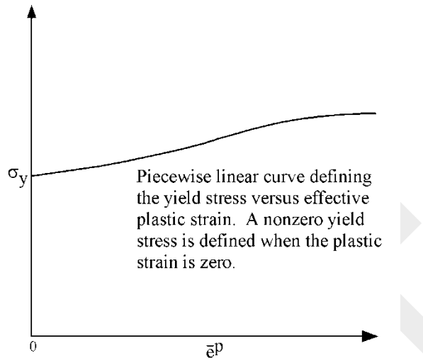
Figure 10.1. Effective stress versus effective plastic strain curve.
