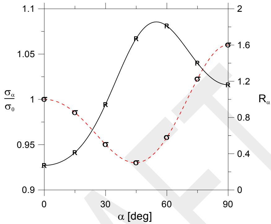
Figure 135.2. Predicted directional variation of the yield stress and plastic flow generated from the file 'R_and_S<#>'. DRAFT
